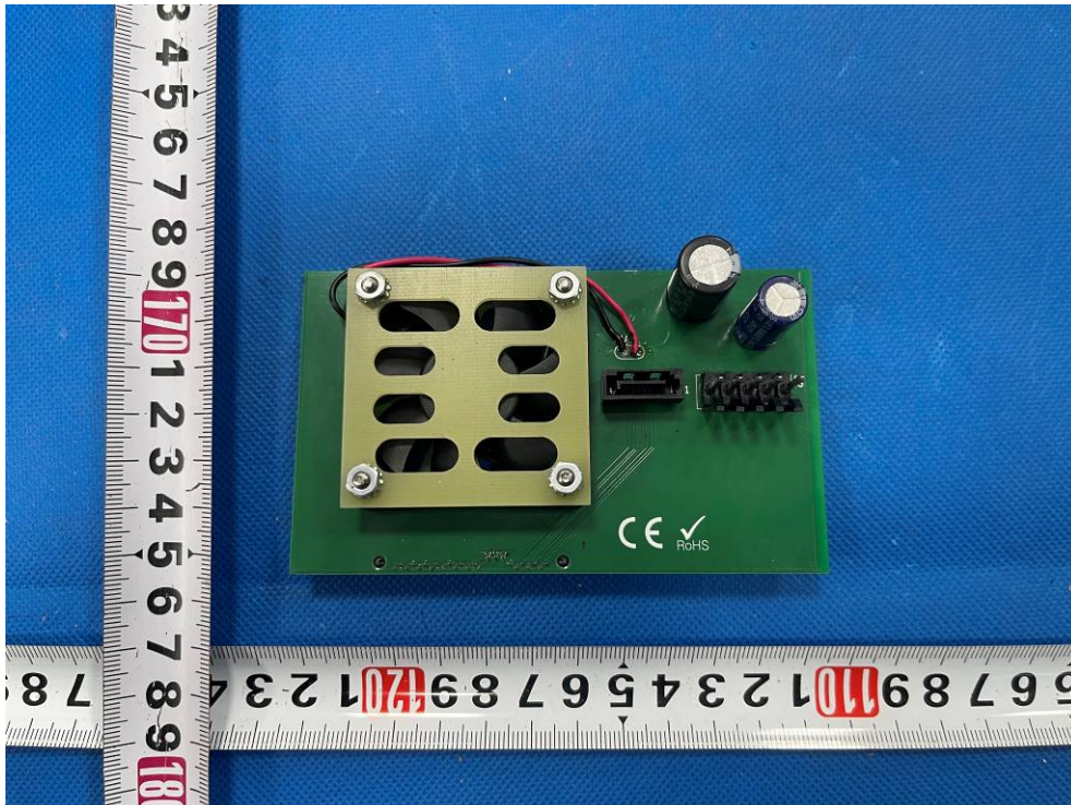
Photo 14: PCB view
